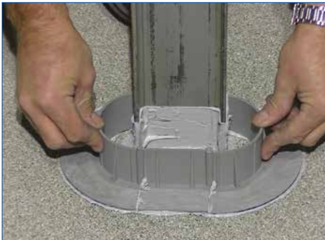
FIGURE 5 - Gluing the POLYSEALANT MOULD formwork
